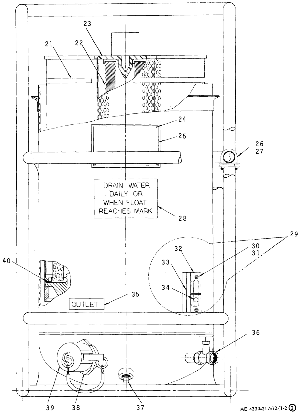
Figure 1-2. Liquid filter separator (sheet 2 of 2).
