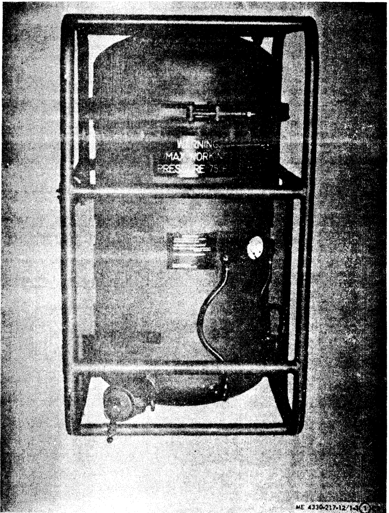
Figure 1-3, Liquid filter-separator (Velcon Model V-1520-ANZ) (sheet 1 of 2).
