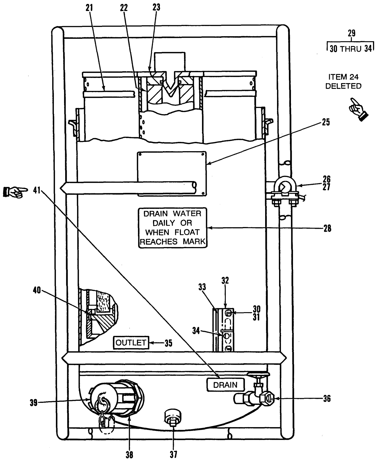
Figure 1-2. Liquid Filter Separator (Sheet 2 of 2).
